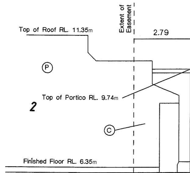
CROSS SECTION 'Y - Y' Not to Scale
